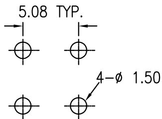
RECOMMEND P.C.B. MOUNT
